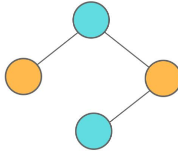
Graph Colouring
